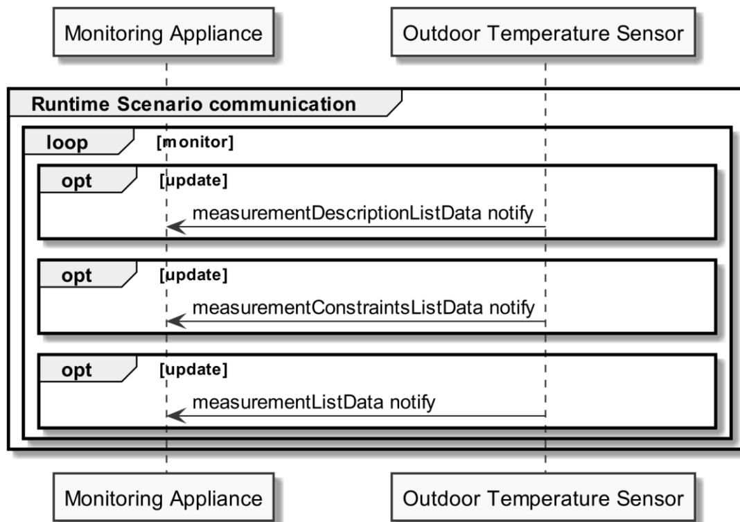
Figure 10: Scenario 1 - Runtime Scenario communication sequence diagram
