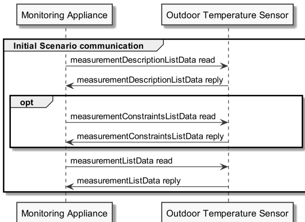
Figure 9: Scenario 1 - Initial Scenario communication sequence diagram
